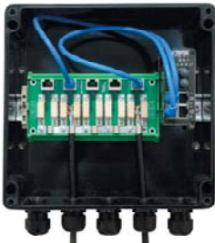
Zone 2 enclosure with LSA modul
